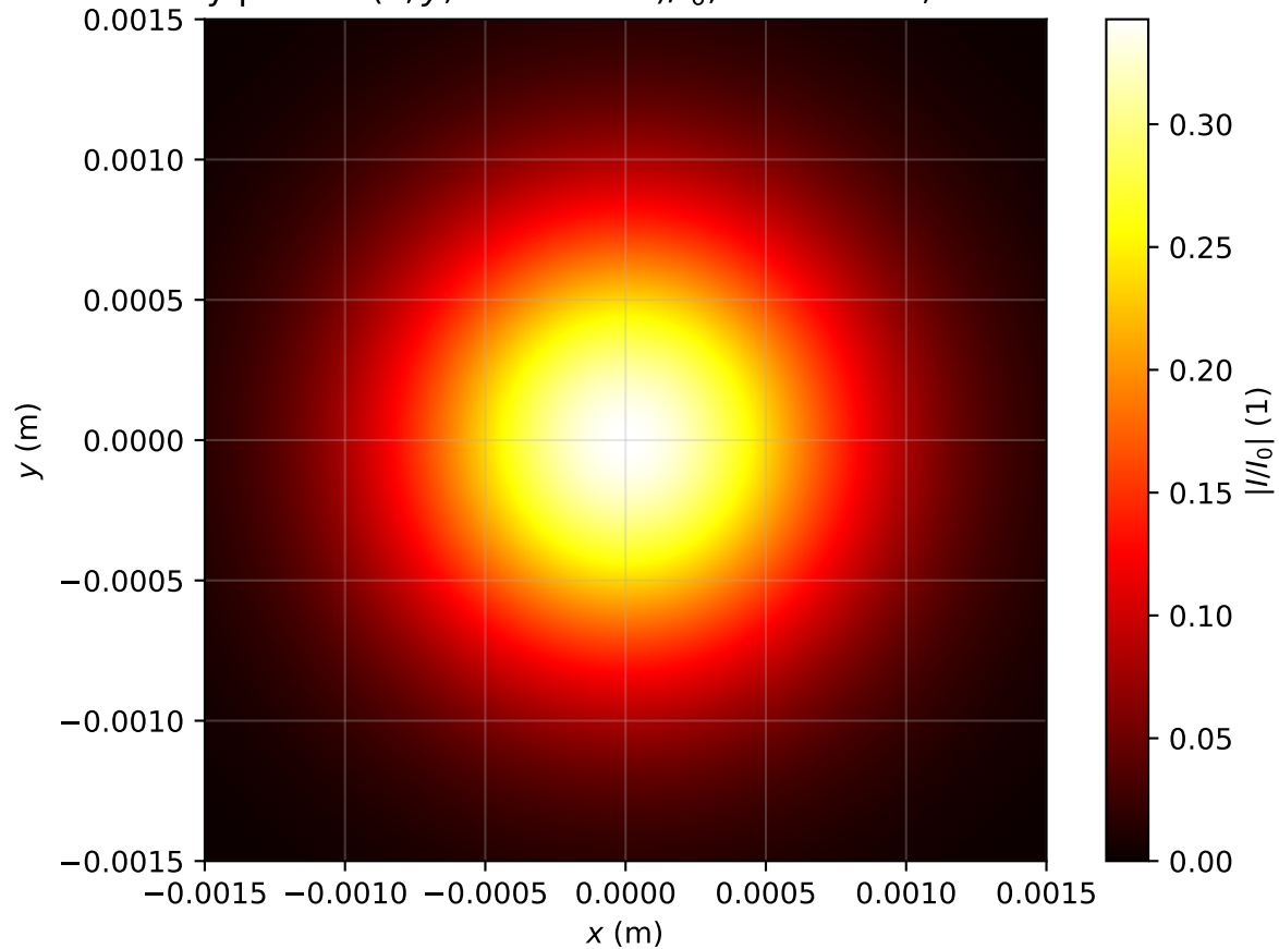
Intensity profile I(x, y, z = 3.503m)/I_0 , P_{in}=0.3P_{cr} , artificial time
